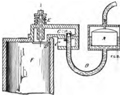
FIG. 312.—Maybach's Original Float Feed Carburetter. A is the hollow float carrying the spindle of the needle valve at its top; B , the tube leading into the inlet valve space; C , the spraying nozzle; D , the inlet valve; E , the inlet valve spring; F , the cylinder space.
